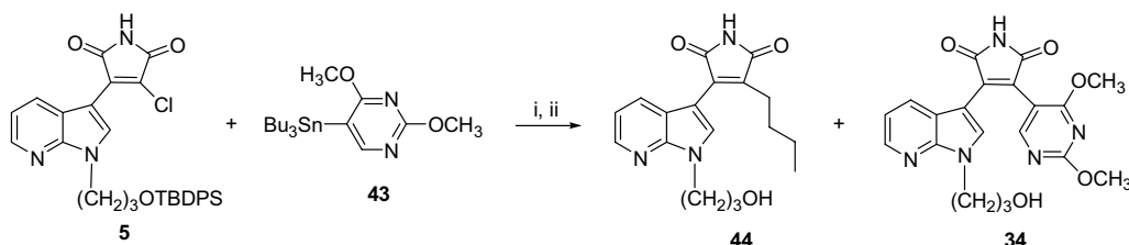
Scheme 7. Reagents and conditions: (i) Pd(P( t -Bu) 3 ) 2 , THF; (ii) TBAF, THF.
