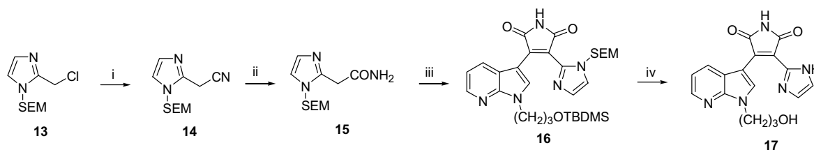
Scheme 4. Reagents and conditions: (i) \text{KCN} , EtOH; (ii) \text{H}_2\text{O}_2 , \text{K}_2\text{CO}_3 , DMSO; (iii) 12, \text{KO}t\text{-Bu} , THF; (iv) TFA, \text{CH}_2\text{Cl}_2 .
