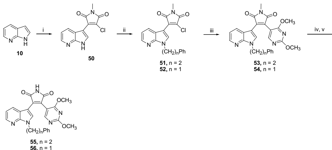
Scheme 8. Reagents and conditions: (i) EtMgBr, 2,3-dichloro- N -methylmaleimide, toluene; (ii) Ph(CH 2 ) n Br, NaH, DMF; (iii) 43 , Pd 2 (dba) 3 , P( t -Bu) 3 , THF/DMF, microwave; (iv) KOH, EtOH, 10% citric acid; (v) HMDS, MeOH/DMF, 80 °C.
