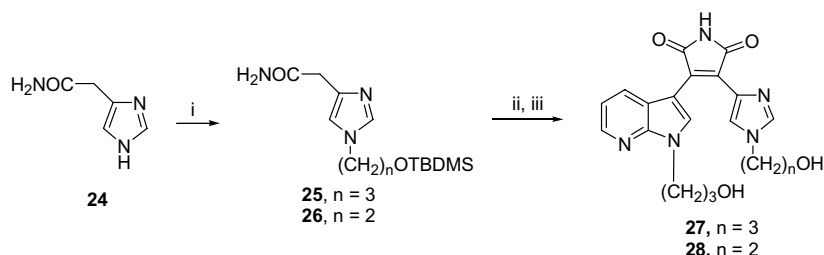
Scheme 6. Reagents and conditions: (i) Br(CH 2 ) n OTBDMS, Cs 2 CO 3 , DMF, 80 °C; (ii) 12 , KO t -Bu, THF; (iii) TBAF, THF.
