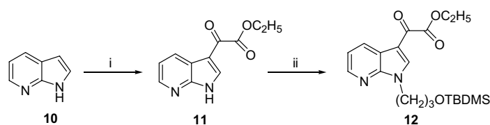
Scheme 3. Reagents and conditions: (i) \text{EtMgBr} , (\text{C}_2\text{H}_5\text{OCO})_2 , THF; (ii) \text{Br}(\text{CH}_2)_3\text{OTBDMS} , \text{Cs}_2\text{CO}_3 , DMF.
