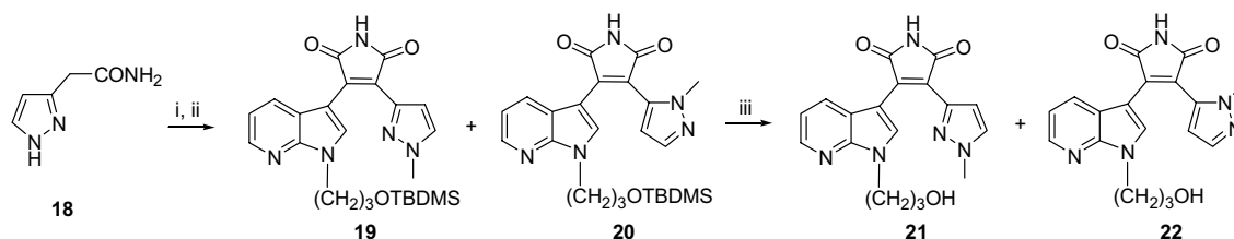
Scheme 5. Reagents and conditions: (i) \text{CH}_3\text{I} , \text{Cs}_2\text{CO}_3 , DMF; (ii) 12, \text{KO}t\text{-Bu} , THF; (iii) TBAF, THF.
