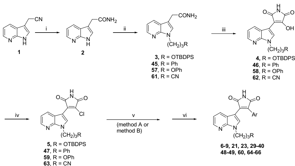
Scheme 2. Reagents and conditions: (i) \text{H}_2\text{O}_2 , \text{K}_2\text{CO}_3 , DMSO; (ii) \text{Br}(\text{CH}_2)_3\text{R} , \text{Cs}_2\text{CO}_3 , DMF; (iii) (\text{CO}_2\text{Et})_2 , \text{KO}t\text{-Bu} , THF; (iv) (\text{COCl})_2 , DMF/ \text{CH}_2\text{Cl}_2 ; (v) method A: \text{Pd}(\text{dba})_3 , \text{Pd}(\text{P}(t\text{-Bu})_3)_2 , \text{ArB}(\text{OH})_2 ; method B: \text{Pd}(\text{P}(t\text{-Bu})_3)_2 , \text{ArSnBu}_3 ; (vi) TBAF, THF (for 5, R = OTBDPS series only).
